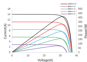
I-V/P-V Curve at Different Irradiation SS8-72HD-545M
